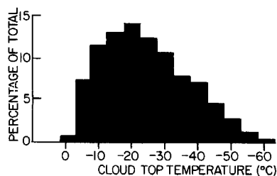
Figure 12. Summary of radar-derived cloud top temperatures for precipitating clouds collected by the Israel Meteorological Service from a site near Tel Aviv (after Gagin and Neumann 1974).
