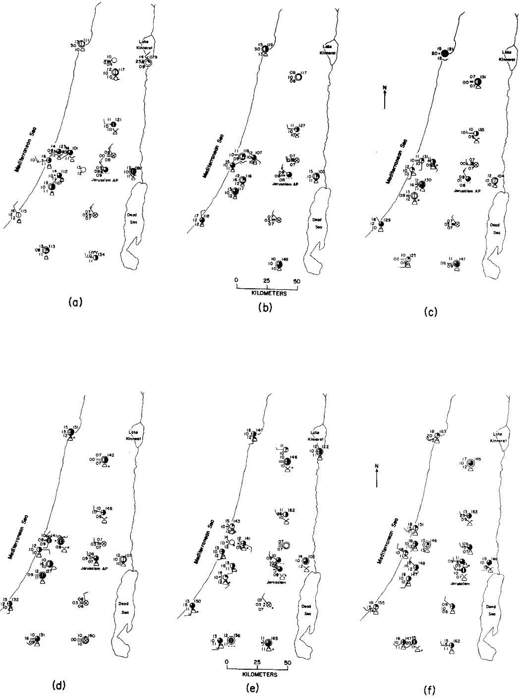
Figure 9. Surface maps for 24 February 1986 at (a) 18 GMT; (b) 21 GMT; and 25 February at (c) 00 GMT; (d) 03 GMT; (e) 06 GMT; and (f) 09 GMT.
