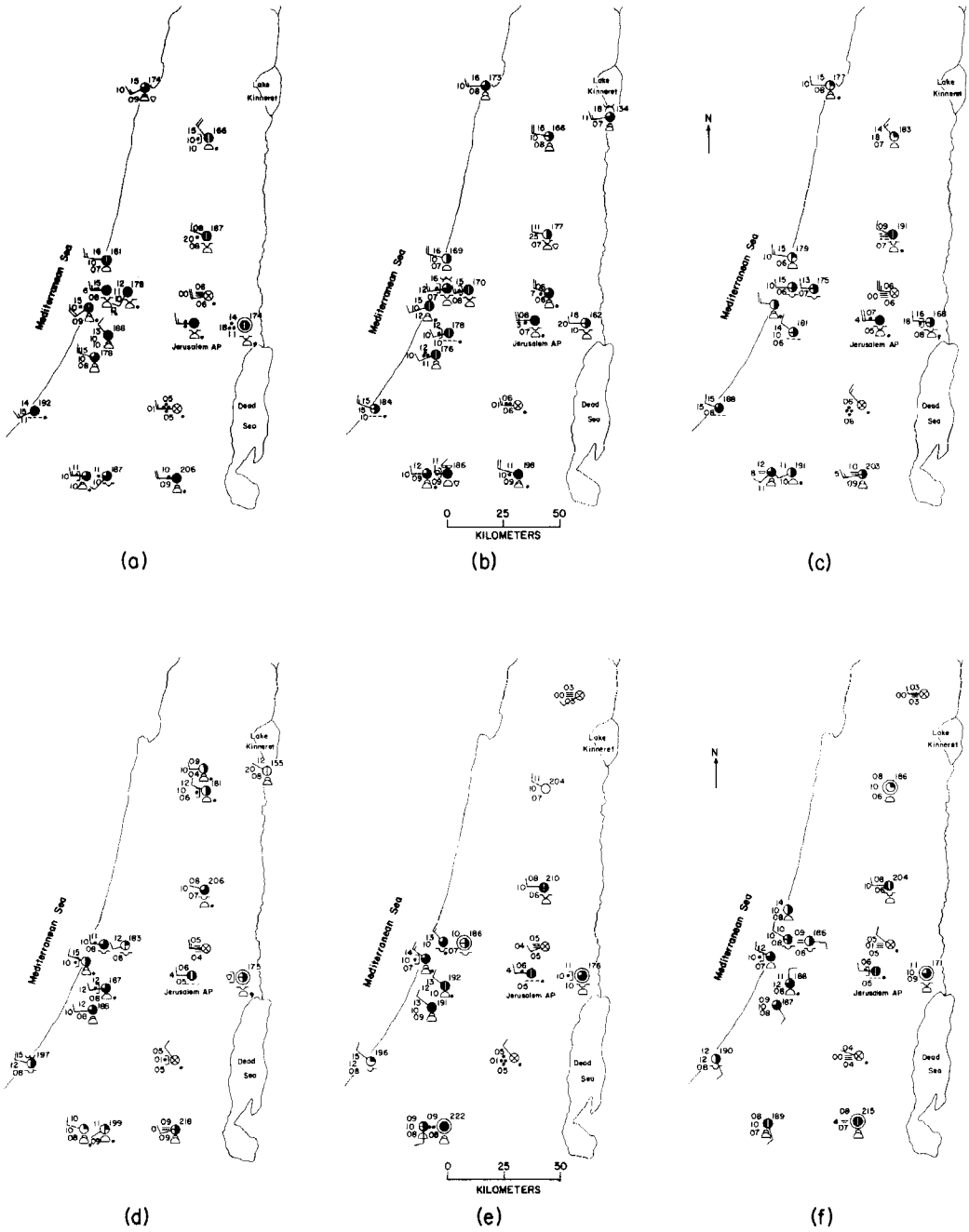
Figure 4. Surface maps for 15 February 1986 at (a) 09 GMT; (b) 12 GMT; (c) 15 GMT; (d) 18 GMT; and (e) 21 GMT; and (f) 00 GMT on 16 February. Standard meteorological symbols have been used.
