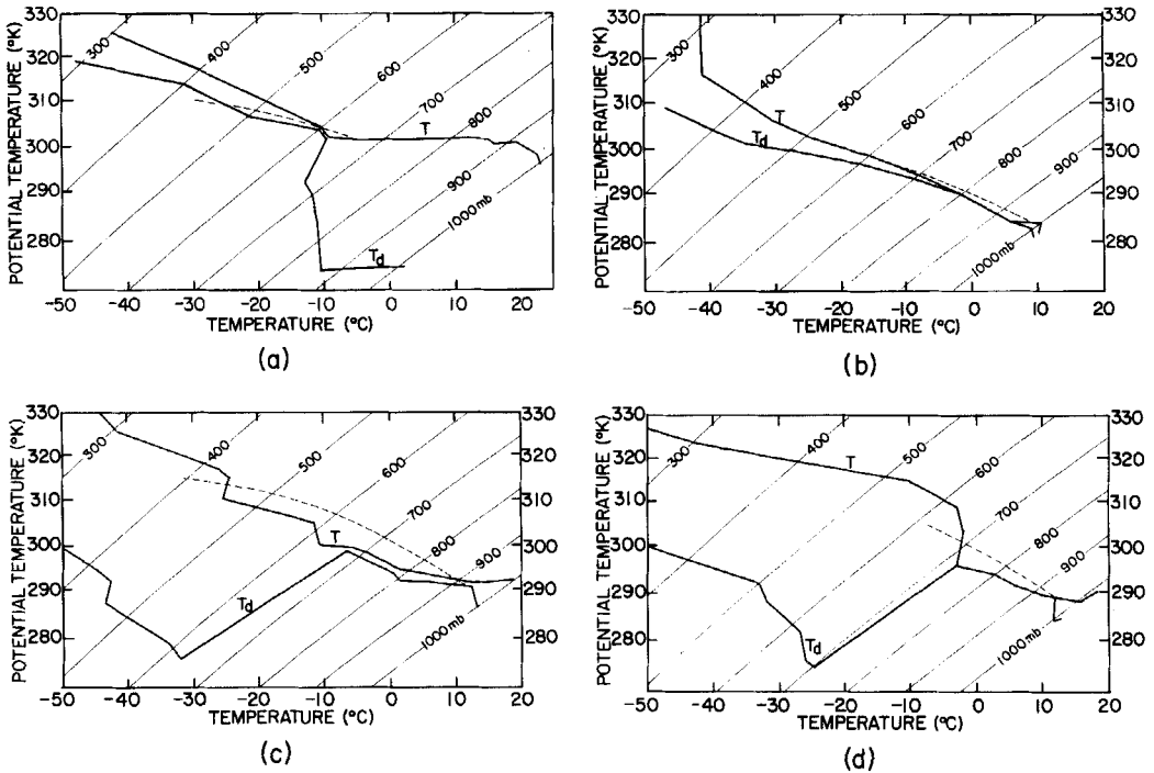
Figure 2. The four types of rawinsonde soundings associated with rain in Israel plotted on a temperature-entropy diagram. (a) Type 2(a), which often precedes frontal passage, is comprised of thick middle- and high-level cloudiness. (b) Type 2(b) is deeply moist and unstable in which thunderstorms often occur. (c) Type 2(c) is highly unstable, but the moisture top is below 600 mb. (d) In type 2(d) the moisture top is below 600 mb and it is capped by a strong stable layer. Pseudoadiabats are indicated by dashed lines, pressure surfaces, in millibars, by sloping fine solid lines and temperature ( T ) and dew-point ( T_d ) soundings by heavy solid lines.
