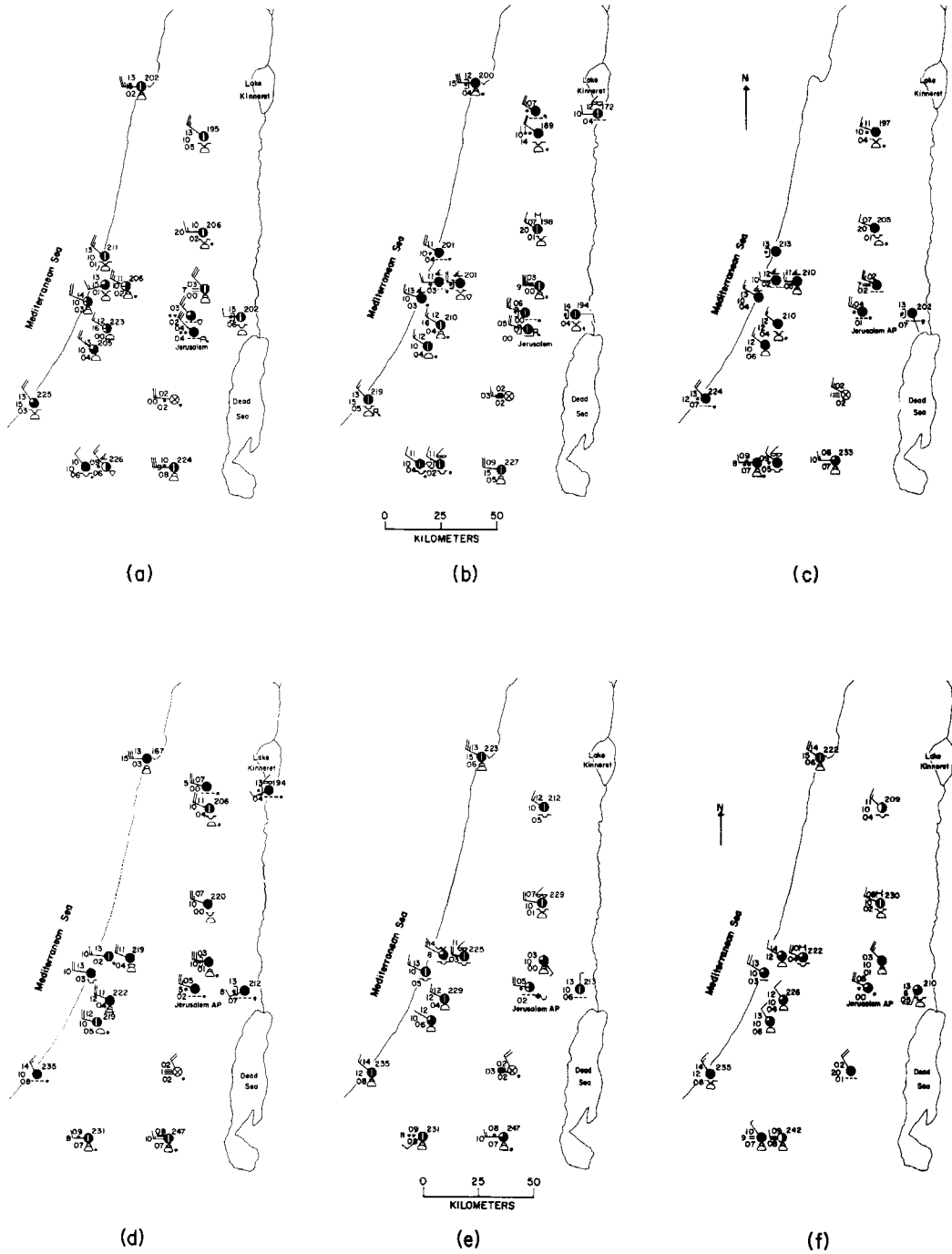
Figure 8. Surface maps for 18 January 1986 at (a) 09 GMT; (b) 12 GMT; (c) 15 GMT; (d) 18 GMT; and (e) 21 GMT; and (f) at 00 GMT on 19 January.
